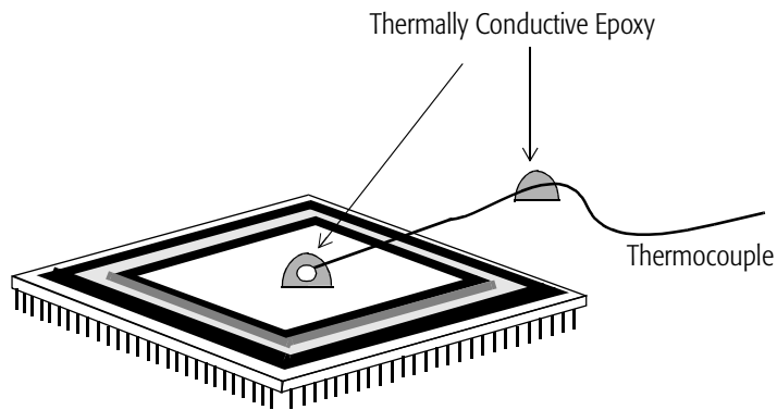
Figure 106. Measuring Case Temperature
