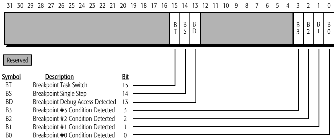
Figure 87. Debug Register DR6
