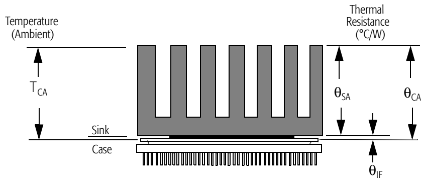
Figure 103. Thermal Model
