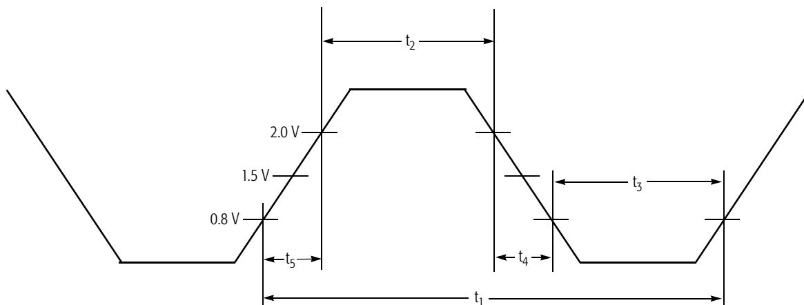
Figure 94. CLK Waveform
