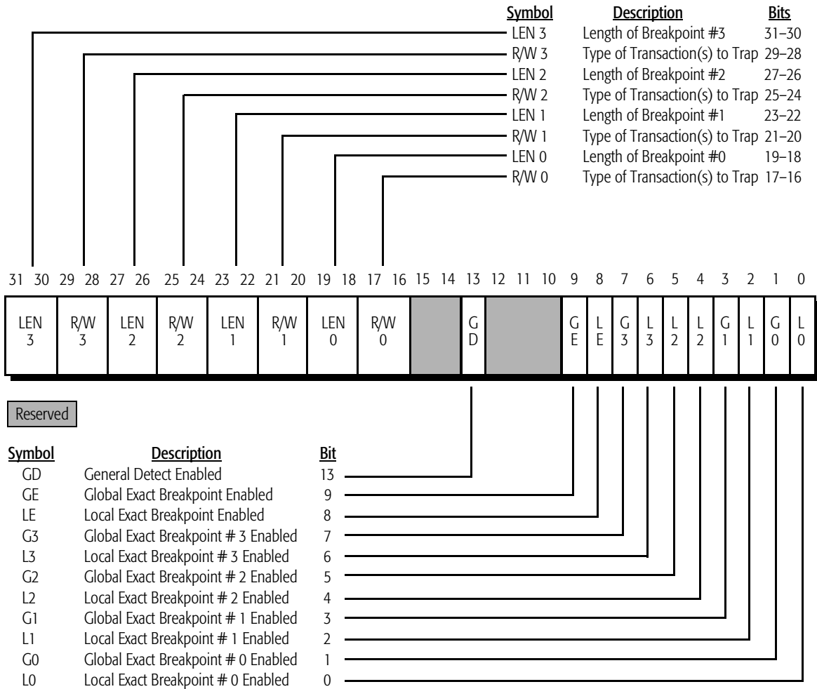
Figure 86. Debug Register DR7
