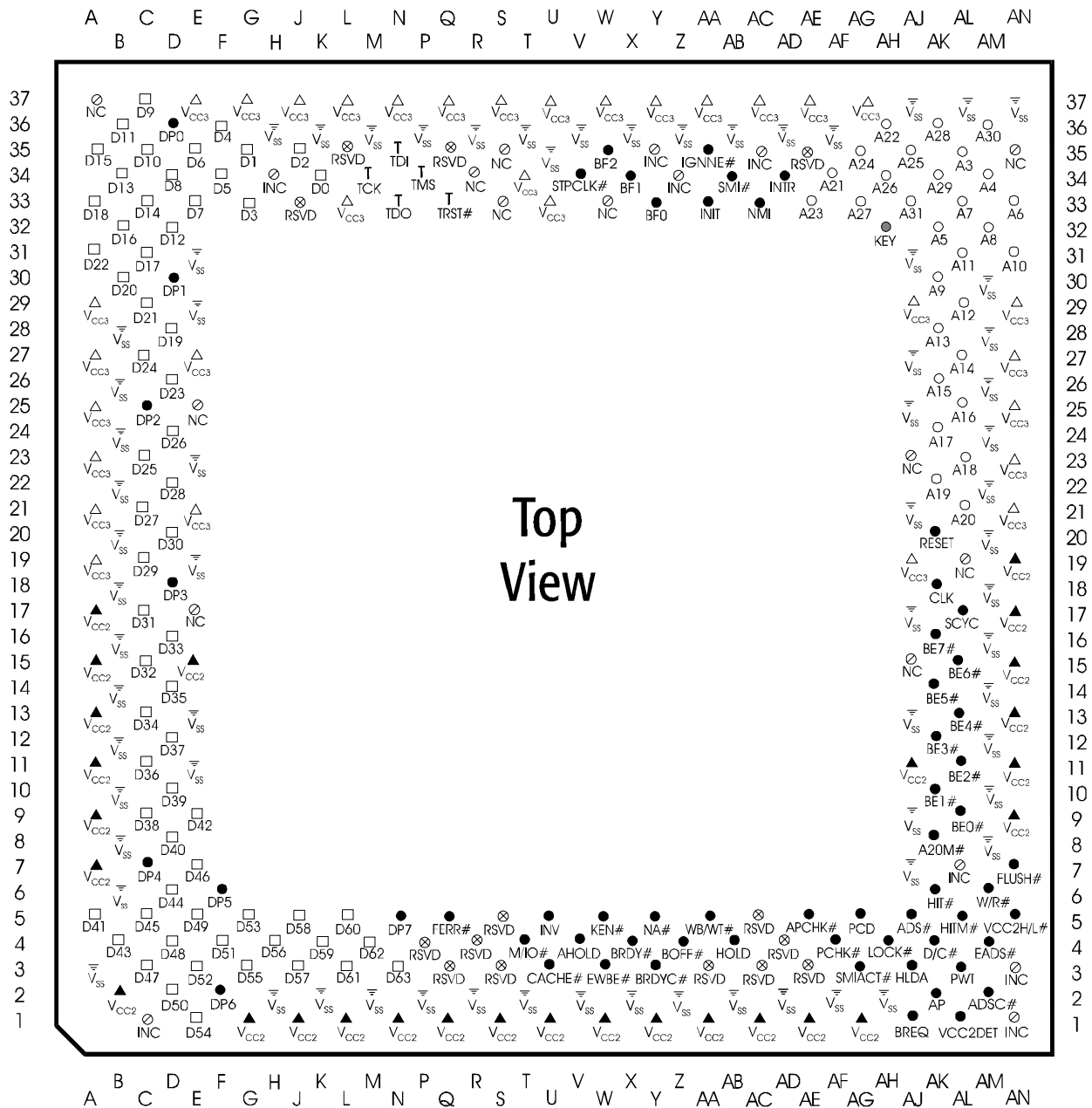
Figure 111. AMD-K6 ® -2 Processor Top-Side View
