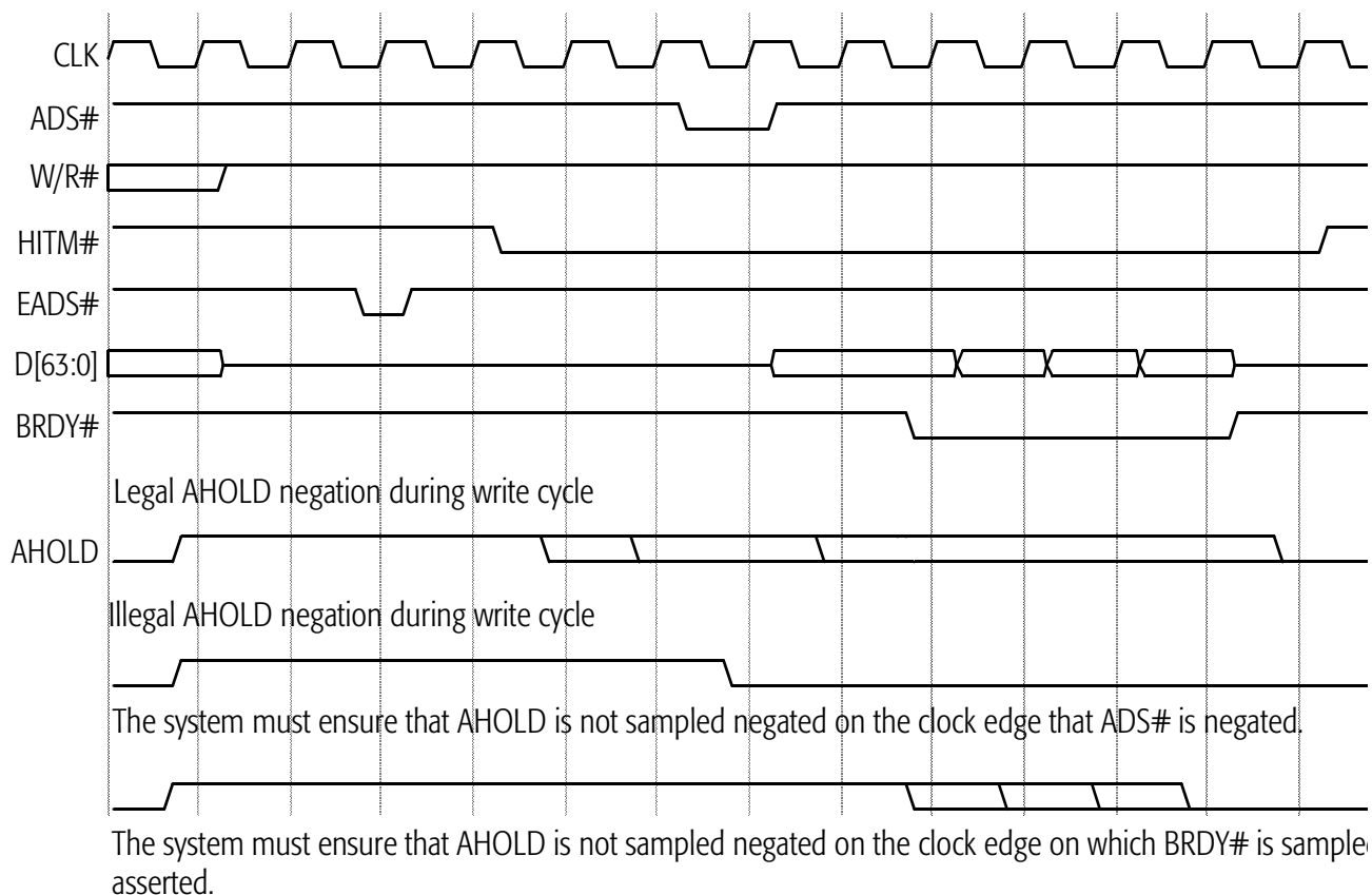
Figure 67. AHOLD Restriction
