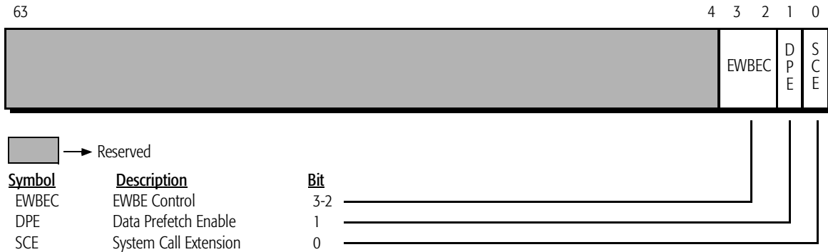
Figure 47. Extended Feature Enable Register (EFER)—Model 8/[F:8]
