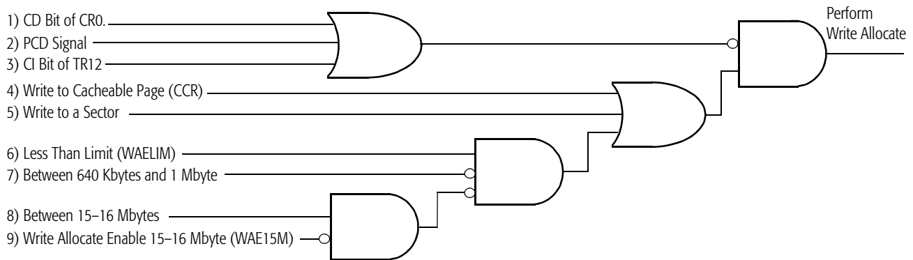
Figure 81. Write Allocate Logic Mechanisms and Conditions
