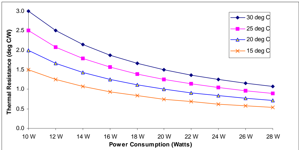
Figure 104. Power Consumption vs. Thermal Resistance
