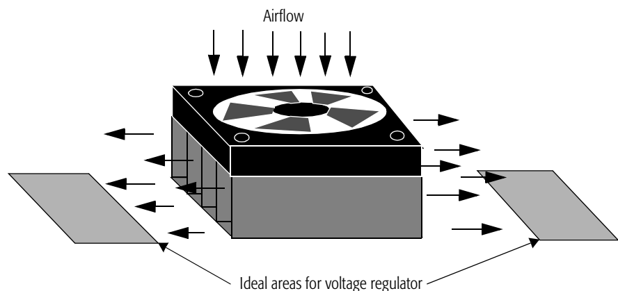
Figure 108. Airflow for a Heatsink with Fan
