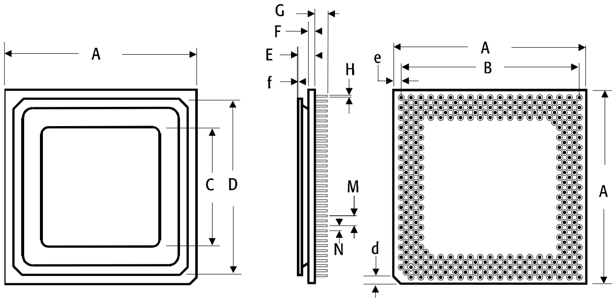
Figure 113. 321-Pin Staggered CPGA Package Specification
