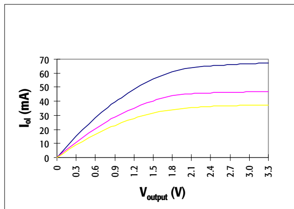
Figure 92. K6STD Pulldown V/I Curves
