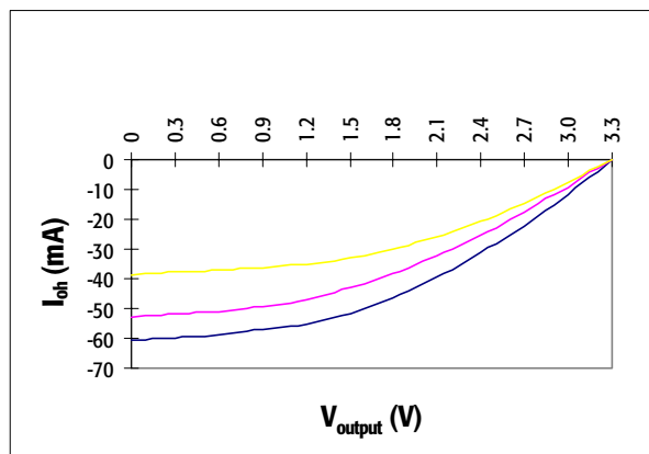
Figure 93. K6STD Pullup V/I Curves
