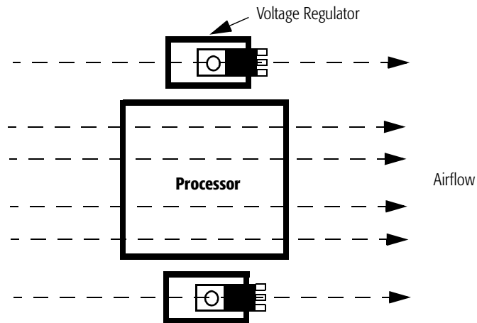
Figure 107. Voltage Regulator Placement
