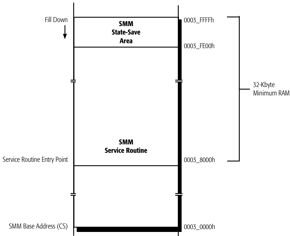
Figure 84. SMM Memory
