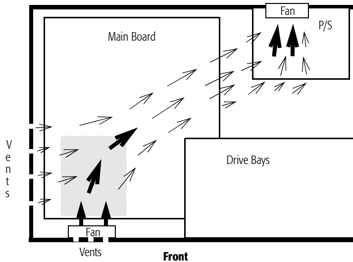
Figure 109. Airflow Path in a Dual-fan System
