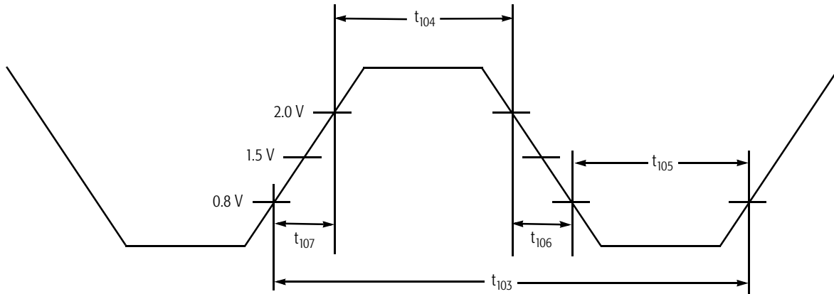
Figure 100. TCK Waveform
