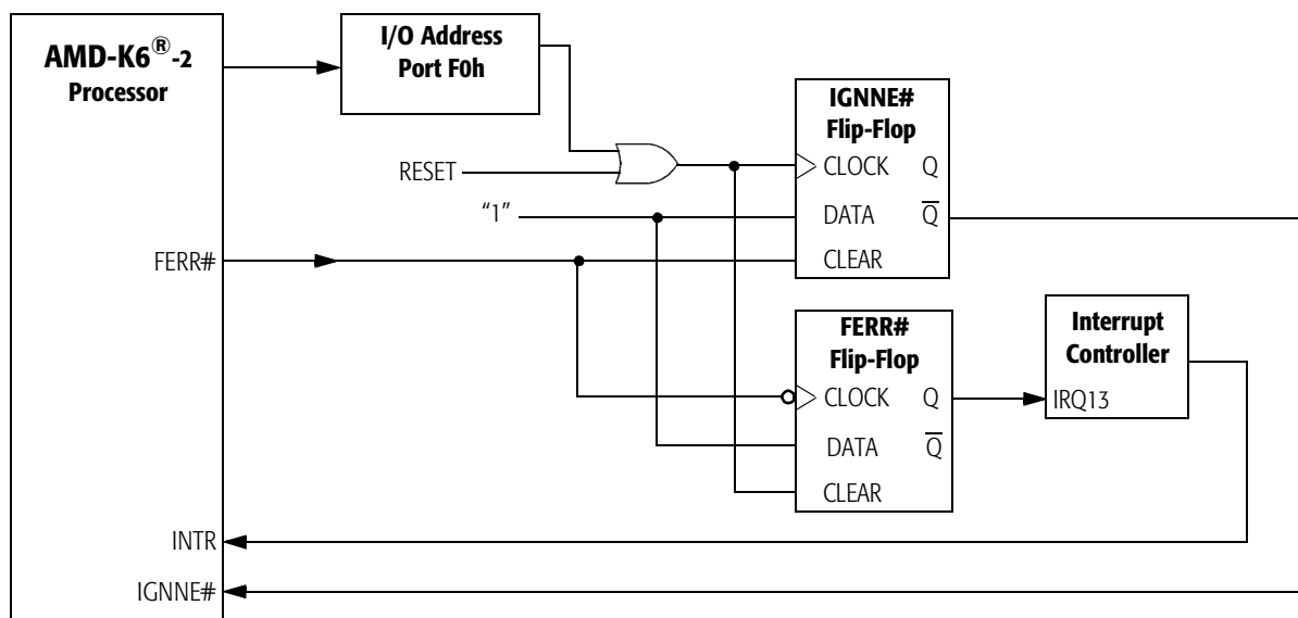
Figure 83. External Logic for Supporting Floating-Point Exceptions
