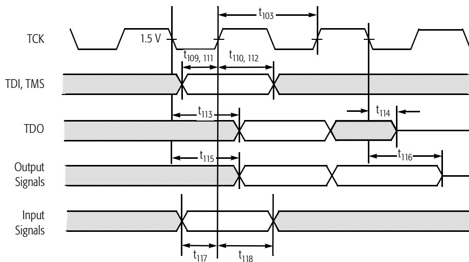
Figure 102. Test Signal Timing Diagram
