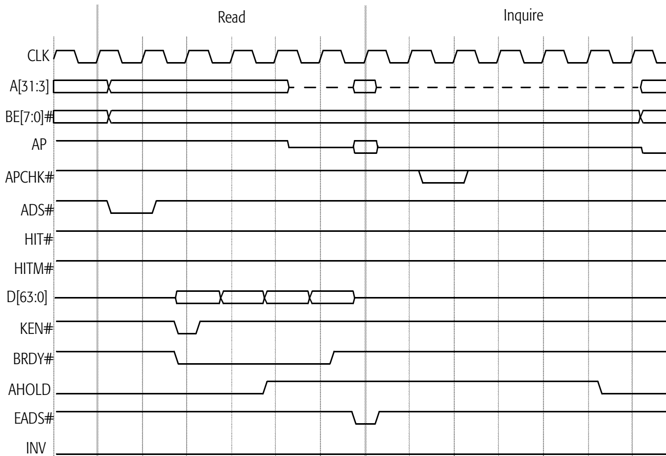
Figure 64. AHOLD-Initiated Inquire Miss
