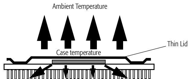
Figure 105. Processor Heat Dissipation Path
