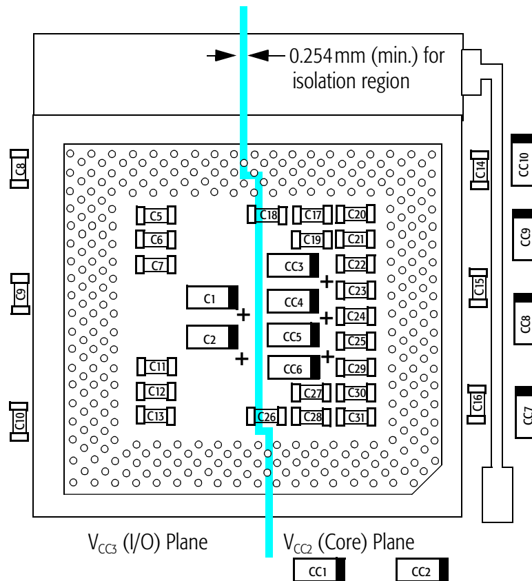
Figure 91. Suggested Component Placement
