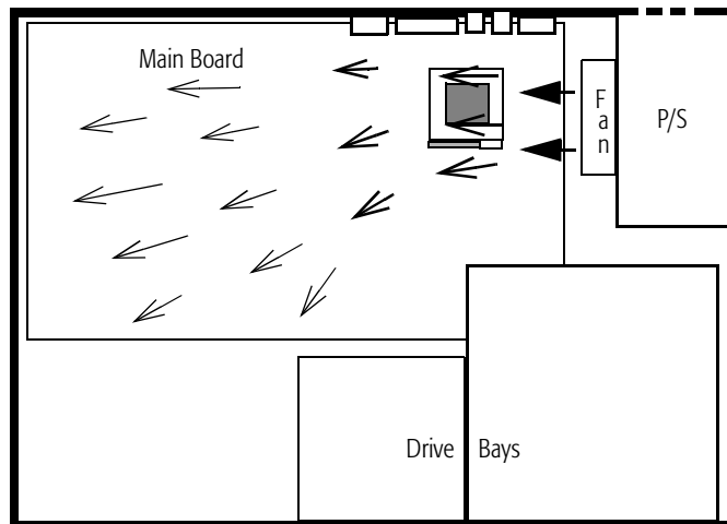
Figure 110. Airflow Path in an ATX Form-Factor System
