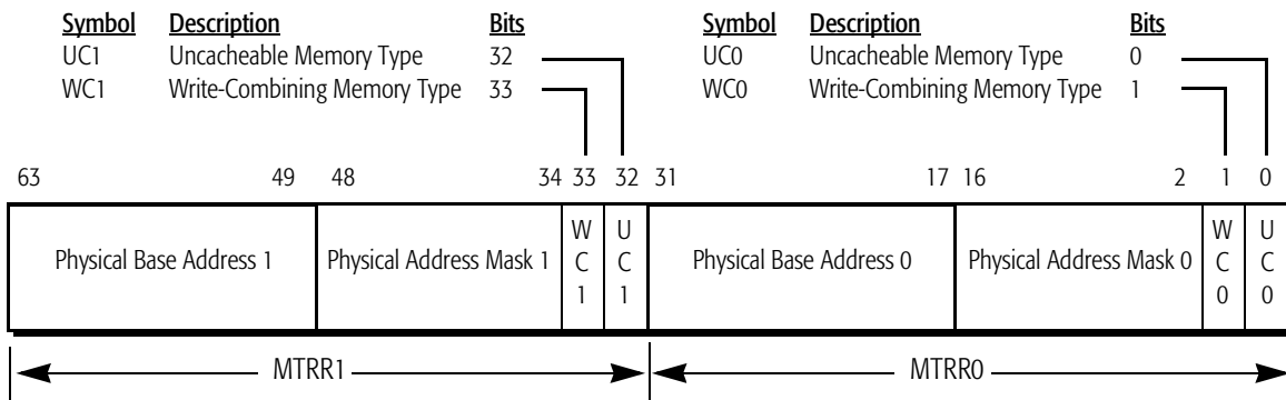
Figure 82. UC/WC Cacheability Control Register (UWCCR)—MSR C000_0085h (Model 8/[F:8])
