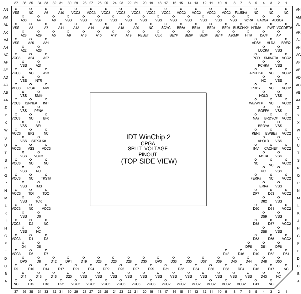
Figure 6-3. CPGA Pinout (Top Side View)
